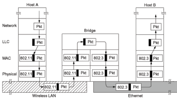
Operation of a LAN bridge from 802.11 to 802.3.
